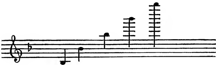
Pitch of the vowels, according to Helmholtz.
